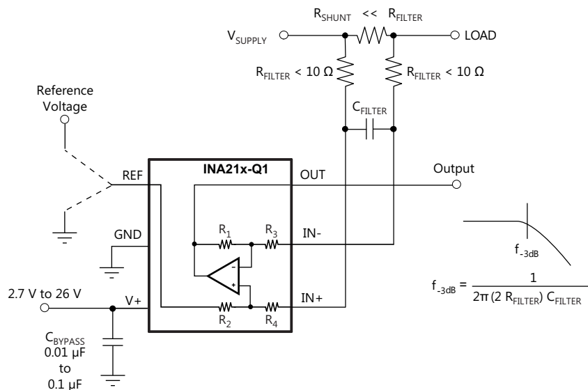
Figure 24. Input Filter
