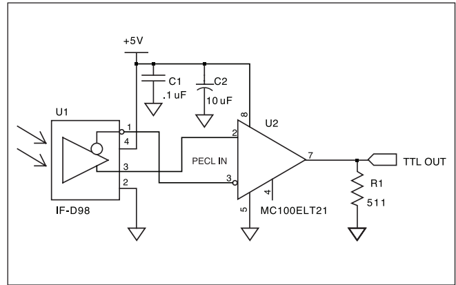
FIGURE 3. Typical interface circuit.
