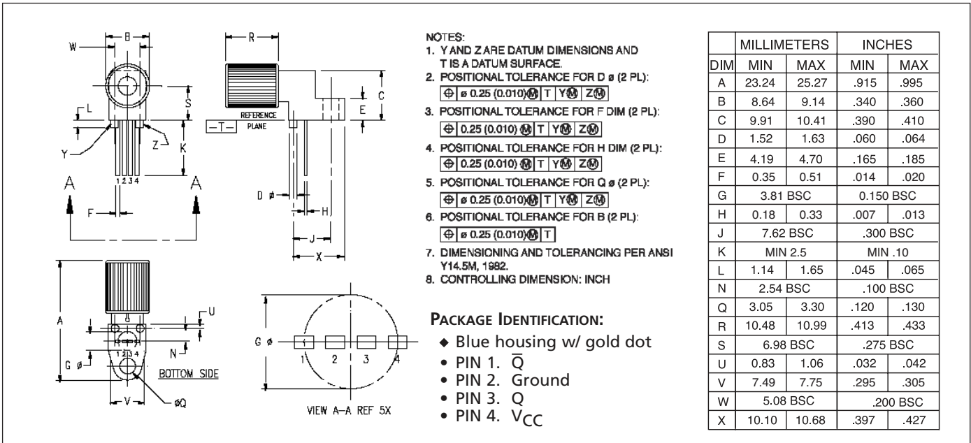
FIGURE 4. Case outline. Specifications are believed to be accurate but are subject to change. Industrial Fiber Optics assumes no responsibility for the consequences of using the information provided beyond replacement warranty for products not meeting stated specifications. Industrial Fiber Optics products are not authorized for use in life support applications without written approval from the President of Industrial Fiber Optics Corporation.
