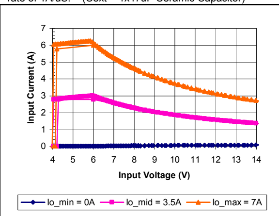
Vo=5V Typical Input Current vs. Input Voltage Characteristic
