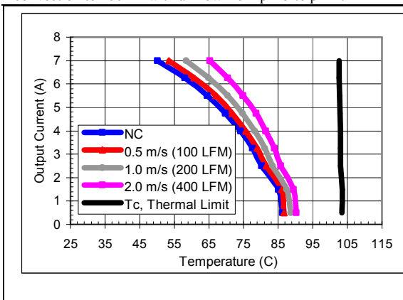
Vo=5V, Vin=12V maximum output current vs. ambient temperature at nominal input voltage for airflow rates natural convection to 400lfm with airflow from pin 5 to pin 1.
