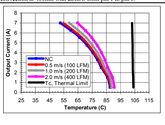
Vo=3.3V, Vin=12V maximum output current vs. ambient temperature at nominal input voltage for airflow rates natural convection to 400lfm with airflow from pin 1 to pin 5.
