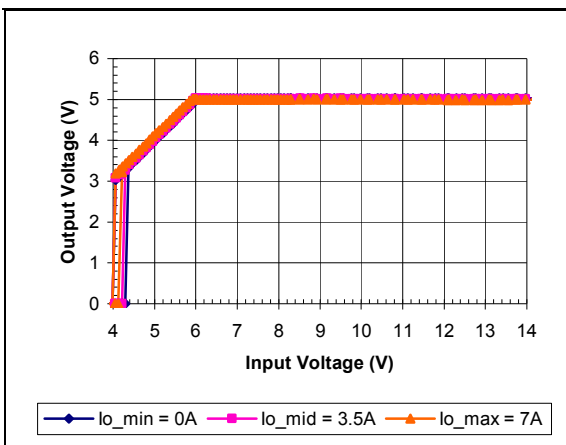
Vo=5V Typical Output Voltage vs. Input Voltage Characteristics
