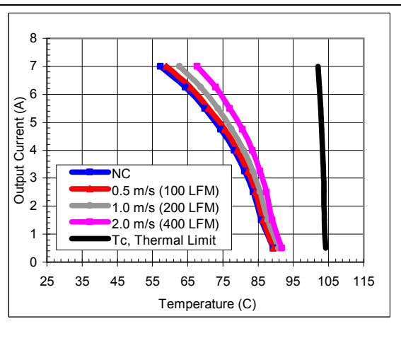
Vo=1.8V, Vin=12V maximum output current vs. ambient temperature at nominal input voltage for airflow rates natural convection to 400lfm with airflow from pin 1 to pin 5.
