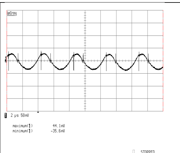
Vo= 3.3V Typical Input Ripple at nominal Input voltage and full load at Ta=25 degrees (Cin = 2x47uF Ceramic Capacitor)
