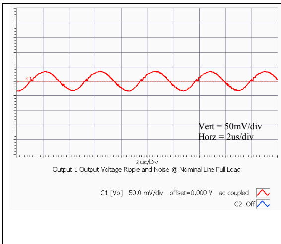
Vo= 5V Typical Output Ripple at nominal Input voltage and full load at Ta=25 degrees (Cext = 1x47uF Ceramic Capacitor)
