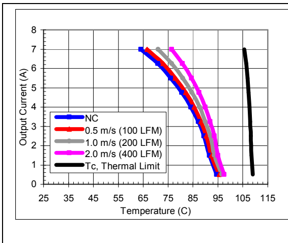
Vo=1.8V, Vin=12V maximum output current vs. ambient temperature at nominal input voltage for airflow rates natural convection to 400lfm with airflow from pin 5 to pin 1.
