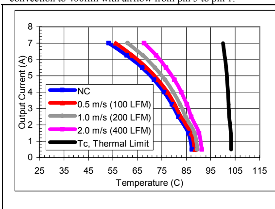
Vo=3.3V, Vin=12V maximum output current vs. ambient temperature at nominal input voltage for airflow rates natural convection to 400lfm with airflow from pin 5 to pin 1.
