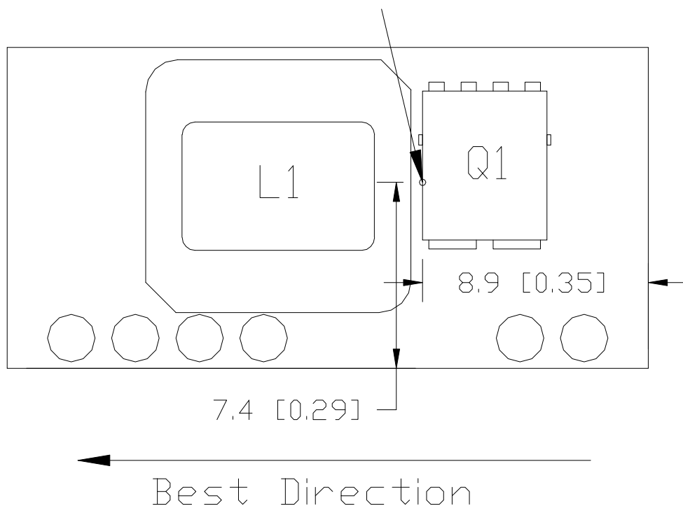
iBD12007A008V thermal measurement location and best airflow orientation
