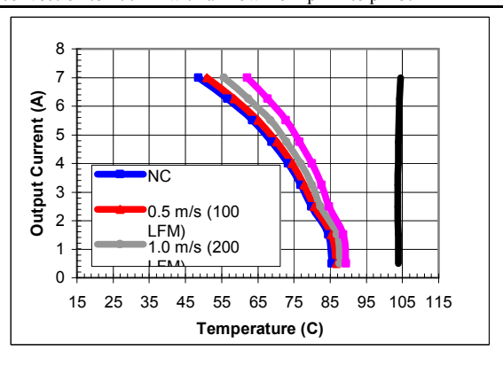
Vo=5V, Vin=12V maximum output current vs. ambient temperature at nominal input voltage for airflow rates natural convection to 400lfm with airflow from pin 1 to pin 5.
