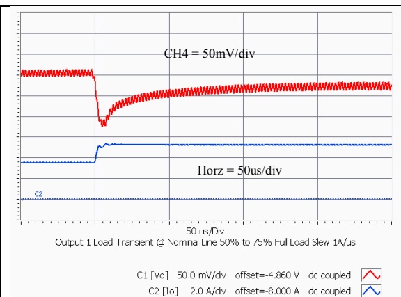
Vo=5V Typical output voltage transient response to load step from 50% to 75% of full load with output current slew rate of 1A/uS. (Cext = 1x47uF Ceramic Capacitor)
