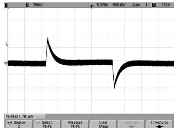
Step Load Transient Response ( V_{in} = 48V , C_{load} = 1\mu F ceramic and 10\mu F tantalum, I_{out} = 50-75-50\% I_{max} , Slew = 0.1A/\mu Sec. , T_a = +25^{\circ}C )
