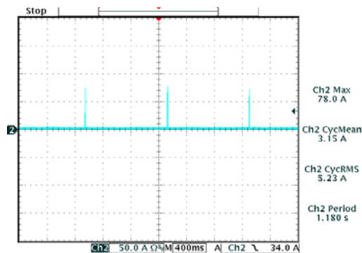
Output Short Circuit Hiccup ( V_{in} = \text{Nom.} , I_{out} = I_{max} , C_{load} = 0 , T_a = +25^{\circ}C )
