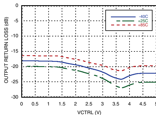
Output Return Loss vs. VCTRL [1]
