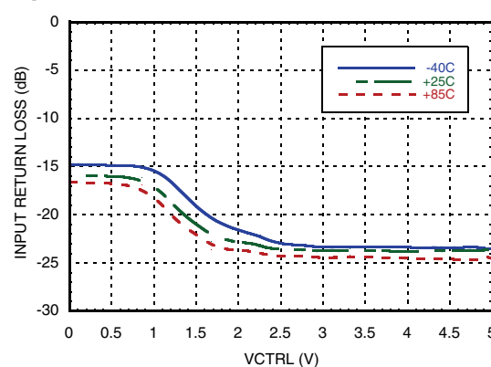
Input Return Loss vs. VCTRL [2]
