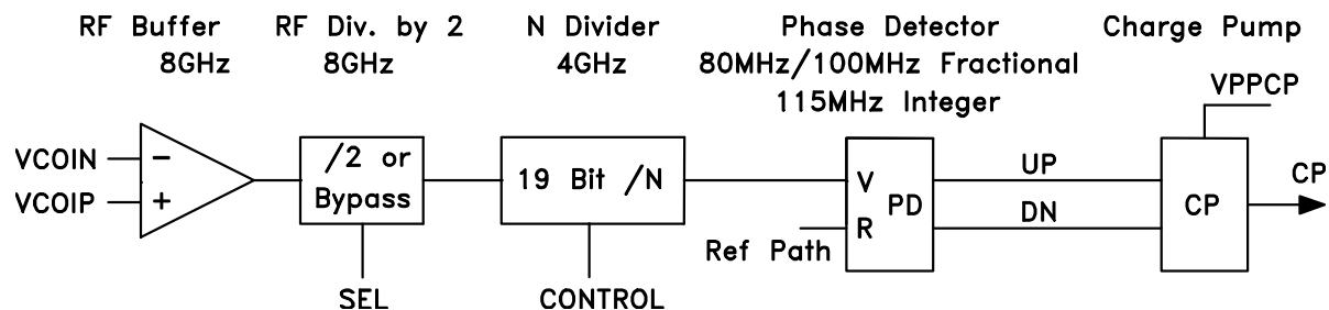
Figure 36. RF Path
