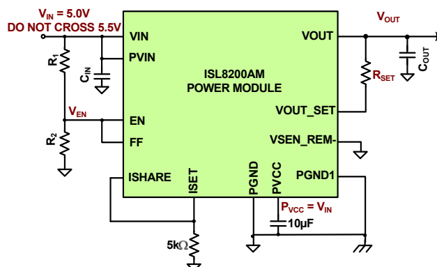
FIGURE 22. 5.0V OPERATION
