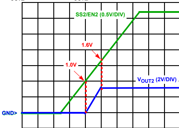
FIGURE 18. SOFT-START
