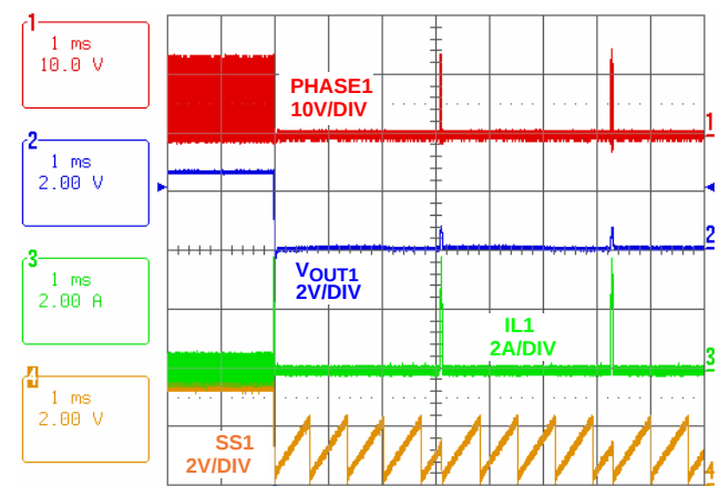
FIGURE 31. POSITIVE OUTPUT SHORT CIRCUIT (HICCUP MODE)
