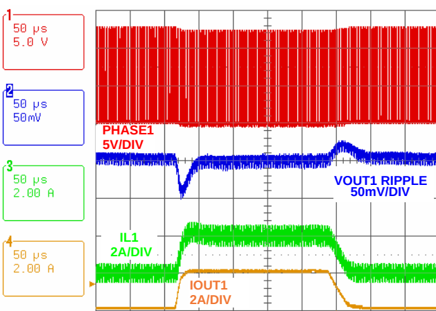
FIGURE 34. LOAD TRANSIENT
