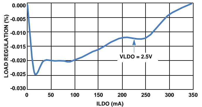
FIGURE 12. LDO LOAD REGULATION vs I_{LD0}
