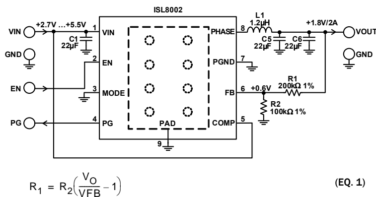
FIGURE 1. TYPICAL APPLICATION CIRCUIT CONFIGURATION (INTERNAL COMPENSATION OPTION)
