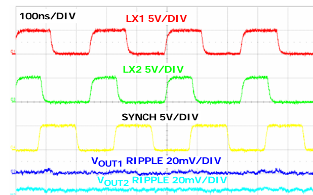
FIGURE 36. CH1 AND CH2 STEADY STATE OPERATION AT NO LOAD (PFM) WITH FREQUENCY = 4MHz
