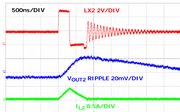
FIGURE 17. STEADY STATE OPERATION AT NO LOAD CHANNEL 2 (PFM)
