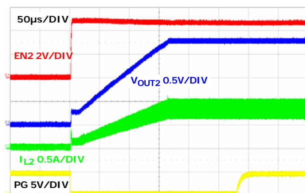
FIGURE 29. SOFT-START AT FULL LOAD CHANNEL 2
