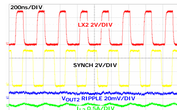
FIGURE 34. CH2 STEADY STATE OPERATION AT NO LOAD (PFM) WITH FREQUENCY = 4MHz
