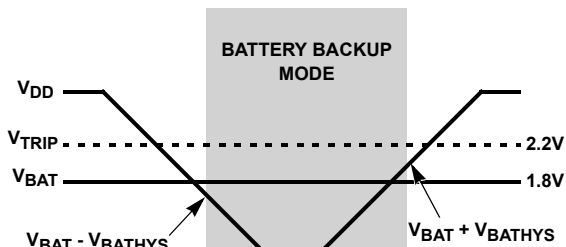
FIGURE 14. BATTERY SWITCHOVER WHEN V_{BAT} < V_{TRIP}
