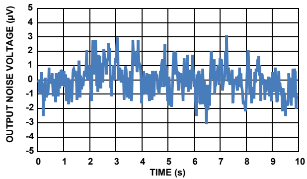
FIGURE 66. V_{OUT} vs NOISE, 0.1Hz TO 10Hz
