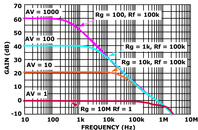
FIGURE 50. SIMULATED FREQUENCY RESPONSE vs CLOSED LOOP GAIN
