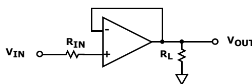
FIGURE 42. INPUT CURRENT LIMITING
