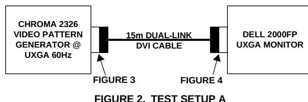
FIGURE 2. TEST SETUP A
