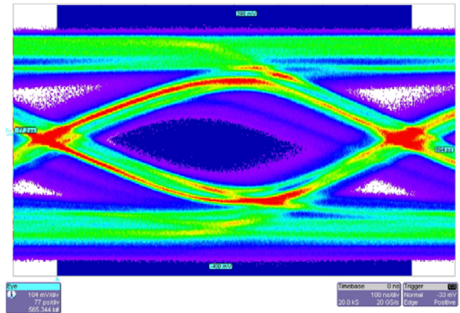
FIGURE 7. ISL54105A EYE DIAGRAM AFTER 15m CABLE
