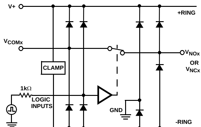
FIGURE 7. OVERVOLTAGE PROTECTION
