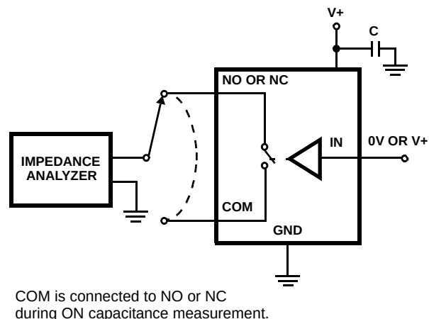
FIGURE 6. CAPACITANCE TEST CIRCUIT
