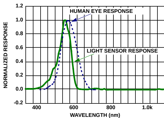
FIGURE 3. SPECTRAL RESPONSE
