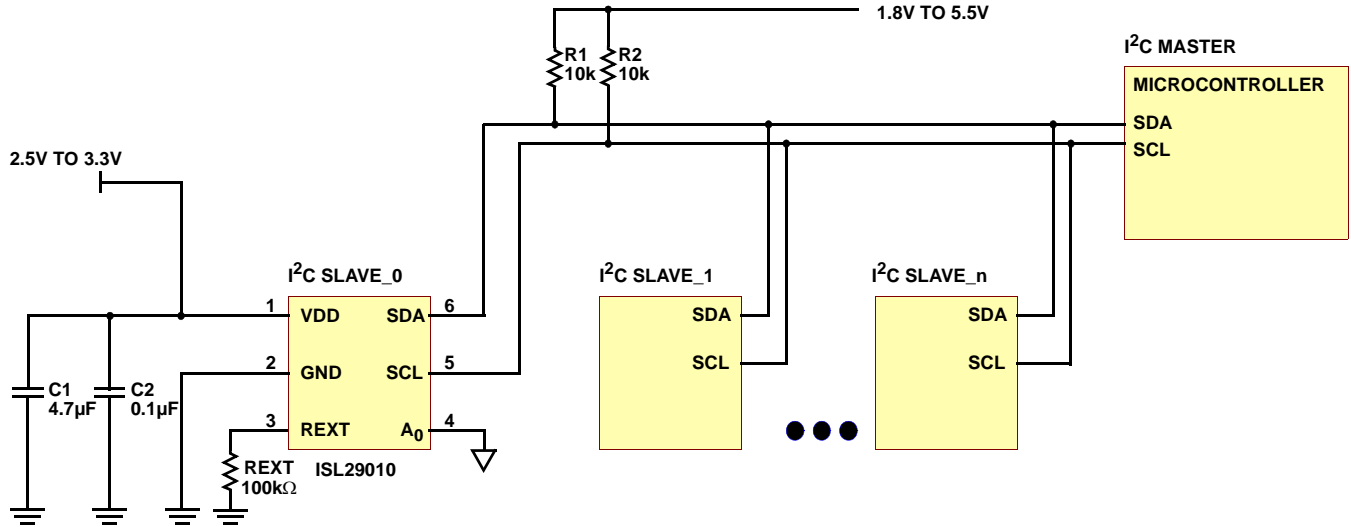
FIGURE 5. ISL29010 TYPICAL CIRCUIT
