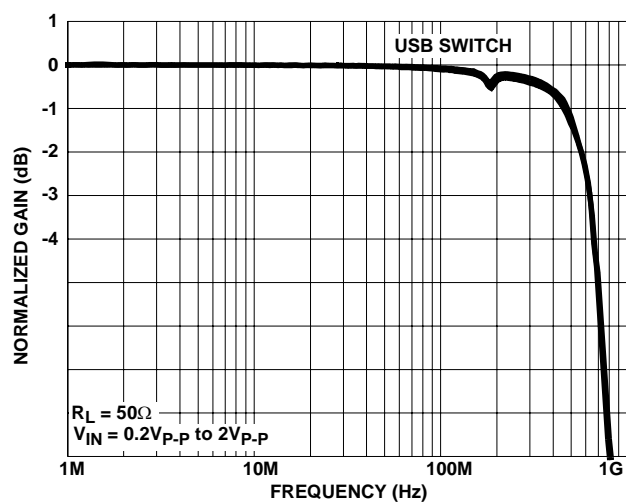
FIGURE 13. FREQUENCY RESPONSE
