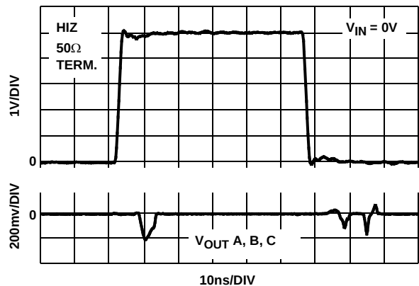
FIGURE 36. MUX 1: HIZ SWITCHING GLITCH V_{IN} = 0V
