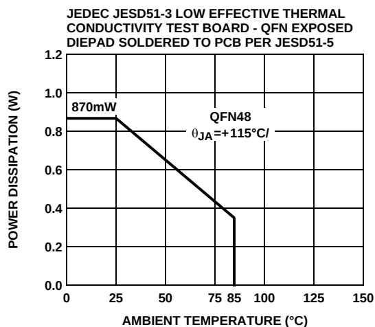
FIGURE 41. PACKAGE POWER DISSIPATION vs AMBIENT TEMPERATURE
