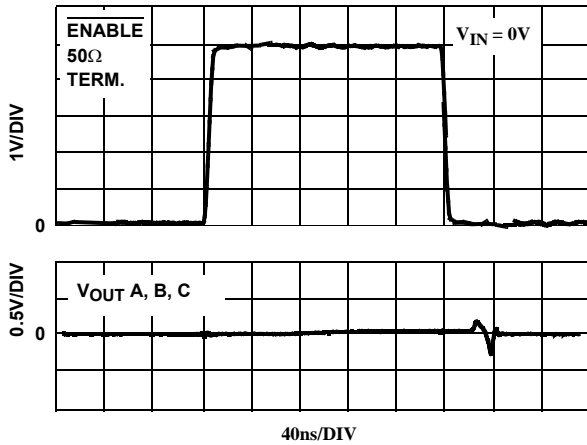
FIGURE 22. ENABLE SWITCHING GLITCH V_{IN} = 0V
