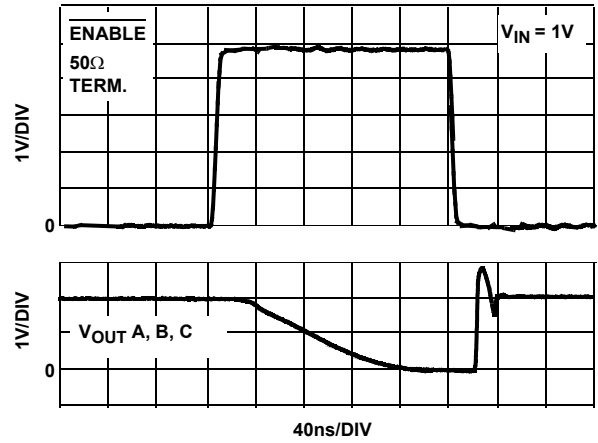
FIGURE 23. ENABLE TRANSIENT RESPONSE V_{IN} = 1V
