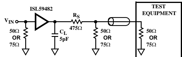
FIGURE 28B. TEST CIRCUIT FOR MEASURING WITH 50Ω OR 75Ω INPUT TERMINATED EQUIPMENT
