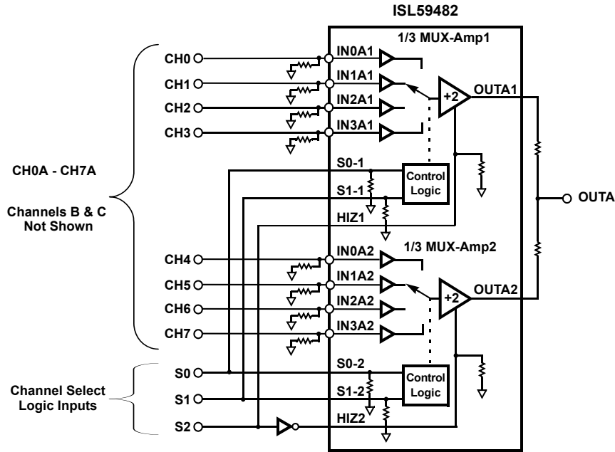
FIGURE 30. APPLICATION CIRCUIT FOR 8:1 RGB VIDEO MUX
