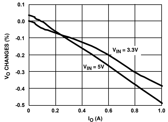
FIGURE 6. LOAD REGULATIONS (PWM MODE)
