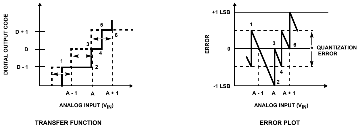
FIGURE 11B. ACCURACY = \pm 1/2 \text{ LSB}
