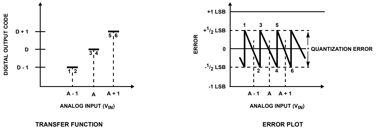
FIGURE 11A. ACCURACY = \pm 0 \text{ LSB} ; PERFECT A/D
