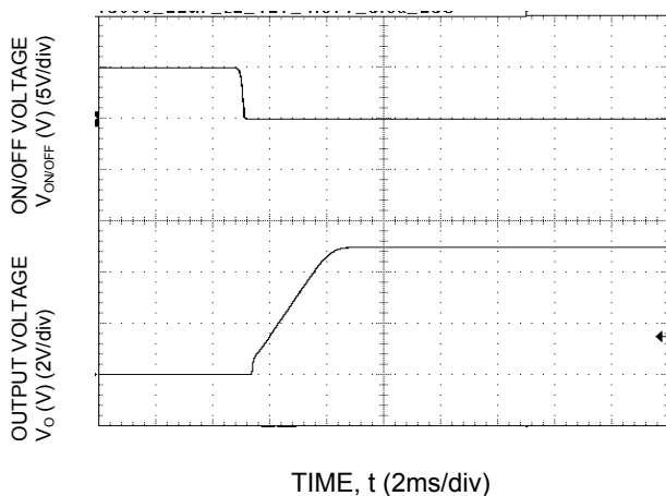
Figure 19. Typical Start-up Using On/Off Voltage (I o = I o,max ).
