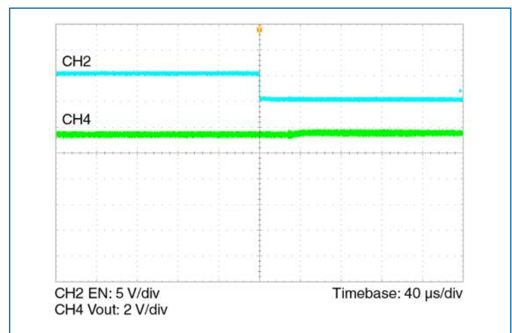
Figure 18 — Three module parallel array test. Vout change with two modules operating and a third module enabled. Nominal Vin, Iout = 140 A
