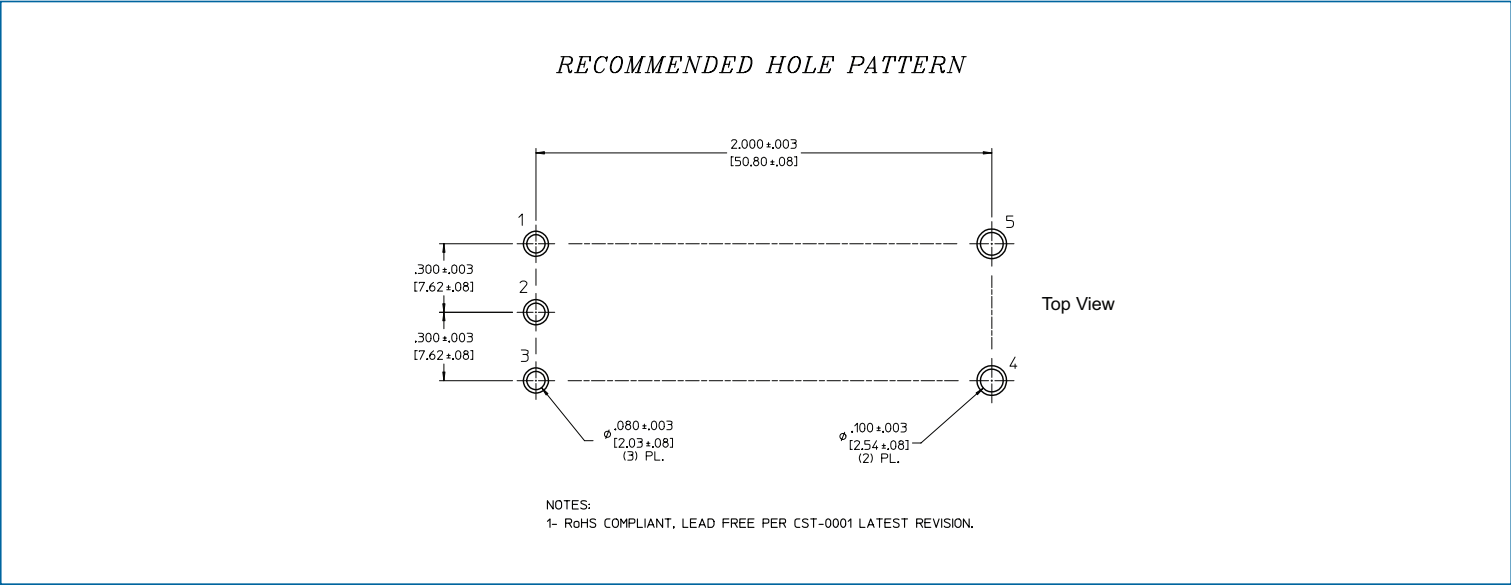
Figure 34 — IBC PCB recommended hole pattern
