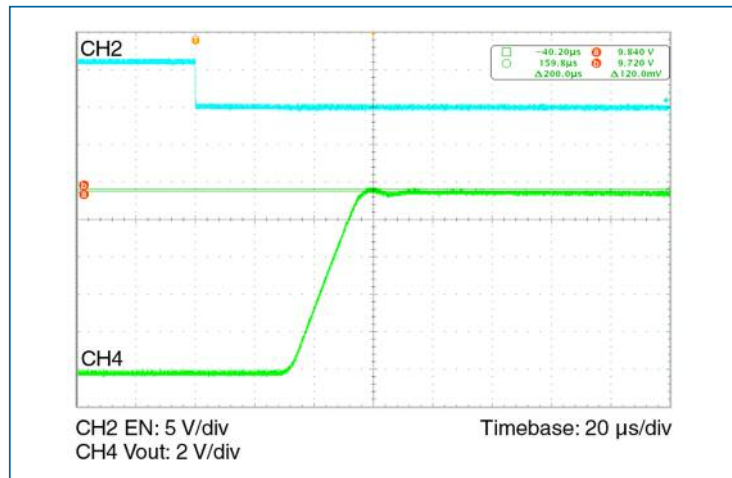
Figure 9 — Overshoot at turn on at nominal line, 15% load 0 load capacitance
