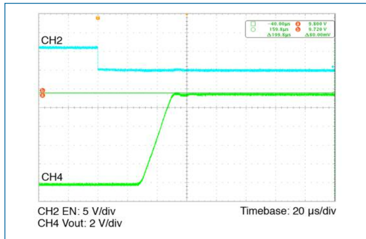
Figure 9 — Overshoot at turn on at nominal line, 15% load
