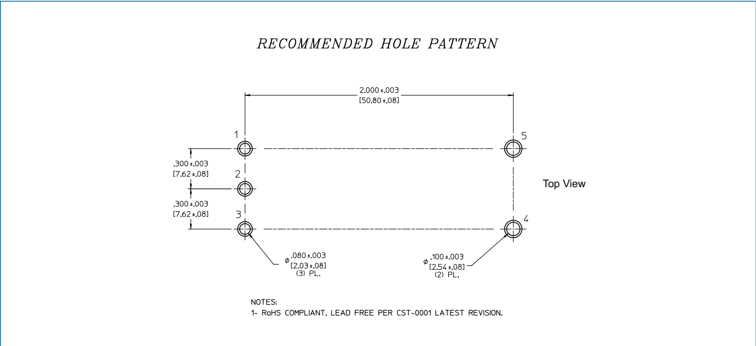
Figure 34 — IBC PCB recommended hole pattern
