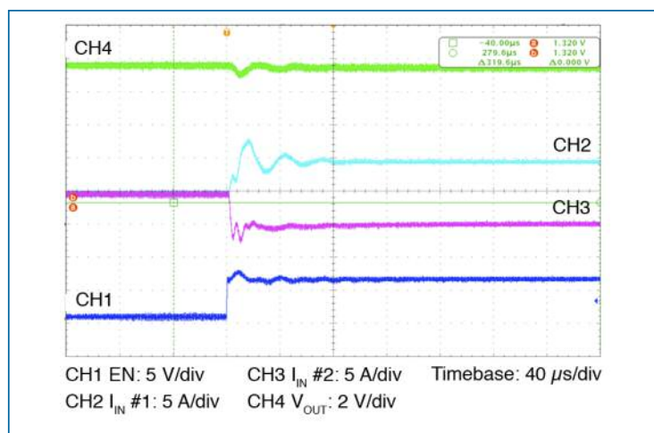
Figure 17 — Two modules parallel array test. Vout and Iin change when one module is disabled. Nominal Vin, Iout = 48A
