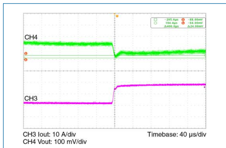
Figure 11 — Load transient response; nominal line Load step 75–100%
