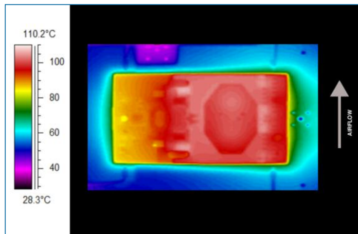
Figure 24 — Thermal plot, 200 LFM, 25°C, 48 Vin, 600 W output power
