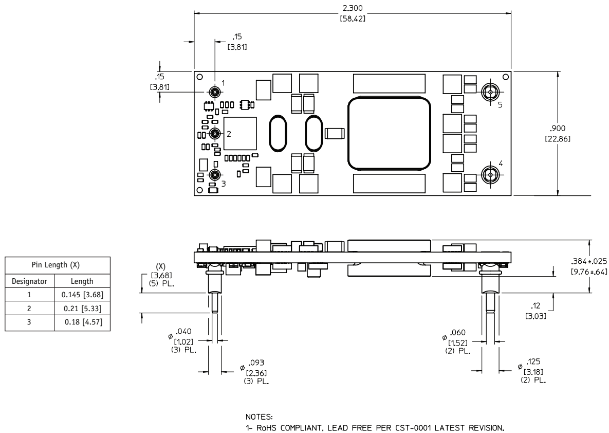
Figure 32 — IBC outline drawing
