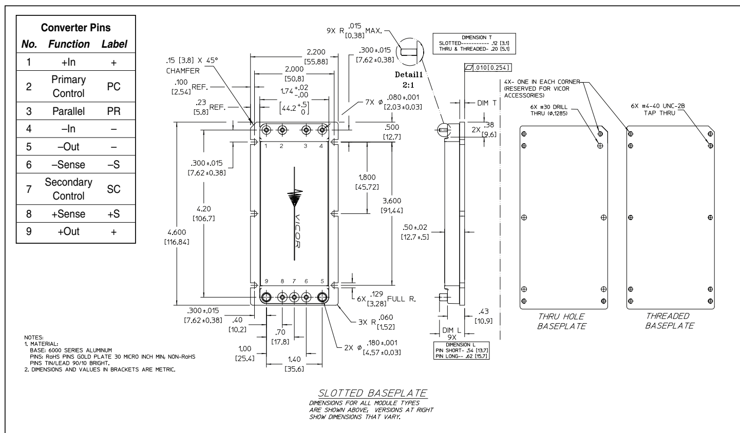
Figure 13 — Module outline
