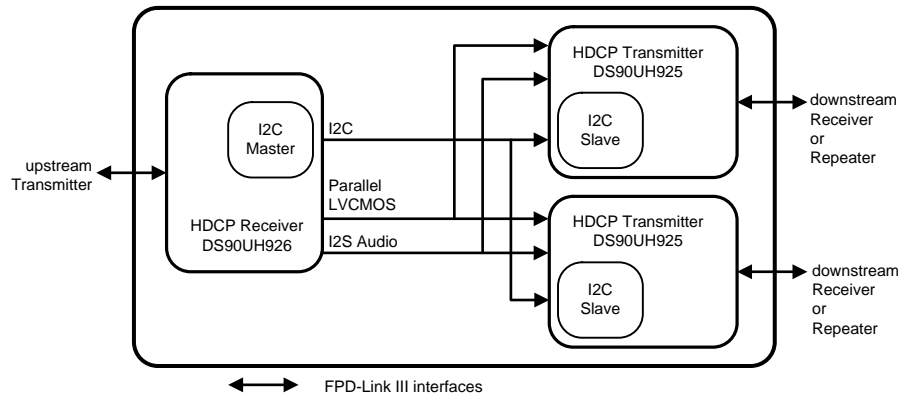
Figure 16. HDCP 1:2 Repeater Configuration
