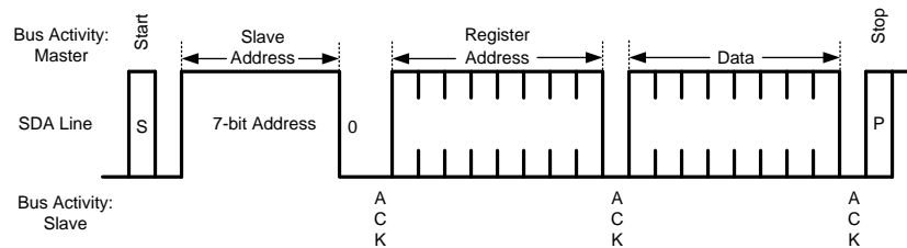
Figure 31. Write Byte
