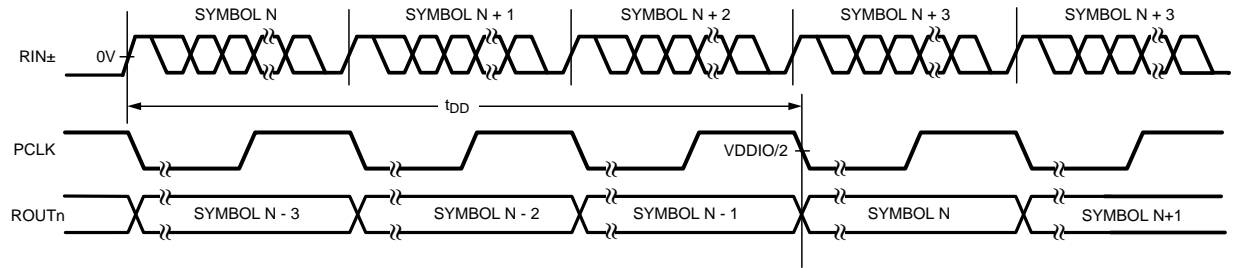
Figure 19. Deserializer Delay
