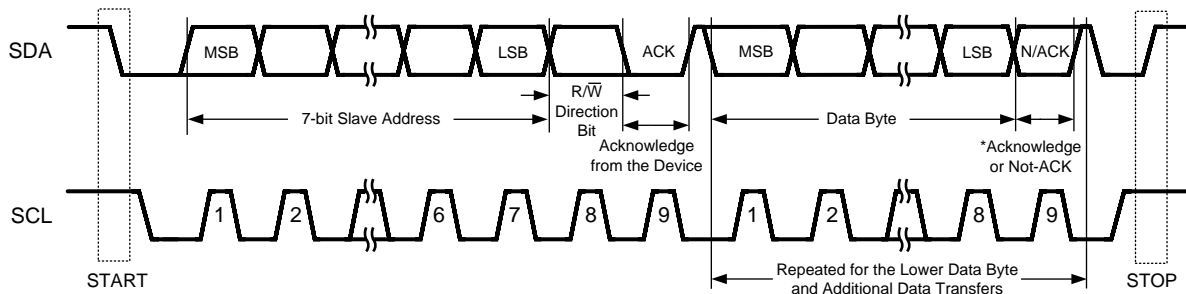
Figure 33. Basic Operation
