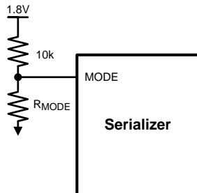
Figure 28. MODE Pin configuration on DS90UB913A-Q1
