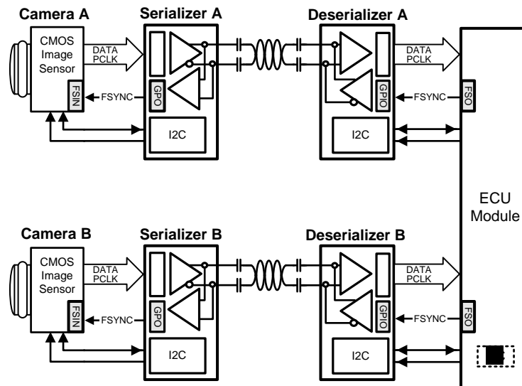
Figure 39. Synchronizing Multiple Cameras
