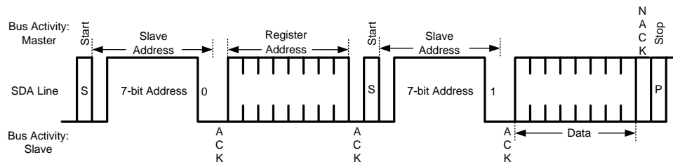
Figure 32. Read Byte
