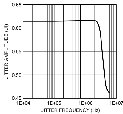
Figure 24. Typical Deserializer Input Jitter Tolerance Curve at 1.4Gbps Line Rate
