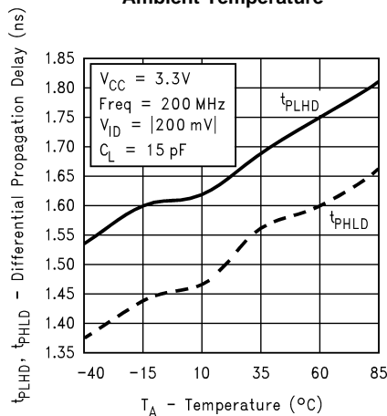
Differential Skew vs Ambient Temperature
