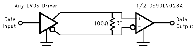
Figure 5. Point-to-Point Application
