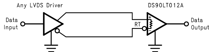
Figure 5. Balanced System — Point-to-Point Application (DS90LT012AQ)
