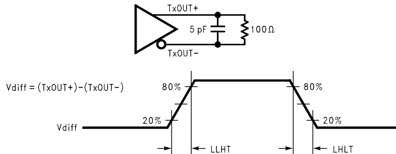
Figure 6. DS90CR213 (Transmitter) Input Clock Transition Time
