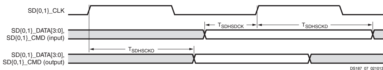
Figure 7: SD/SDIO Interface High Speed Mode Timing Diagram
