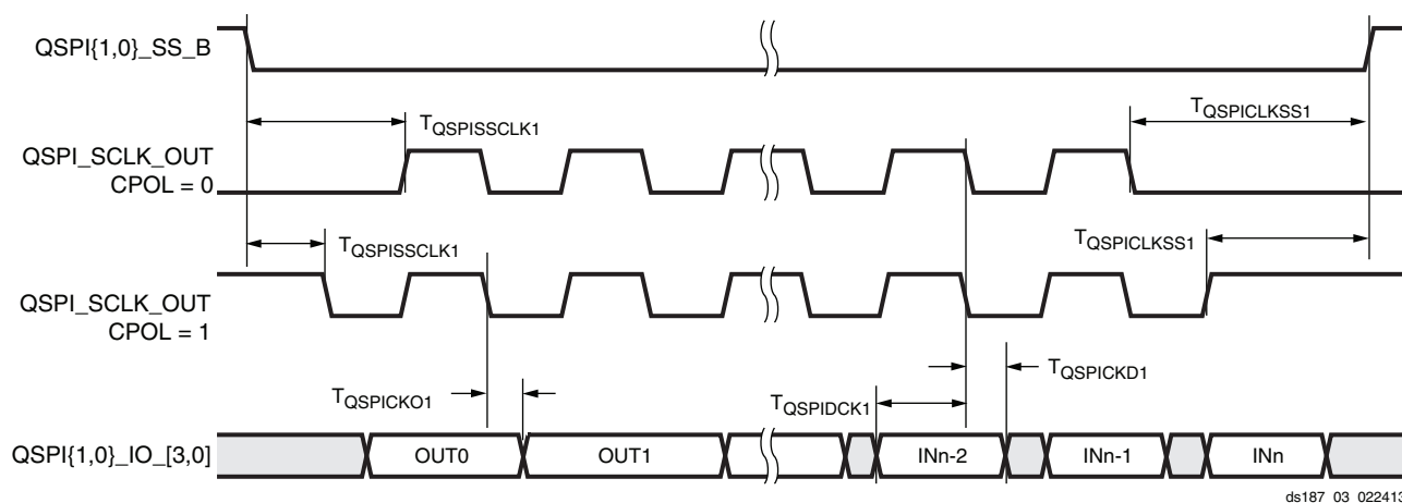
Figure 3: Quad-SPI Interface (Feedback Clock Enabled) Timing Diagram
