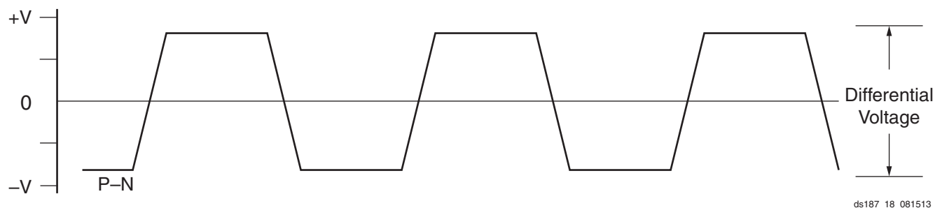
Figure 18: Differential Peak-to-Peak Voltage
