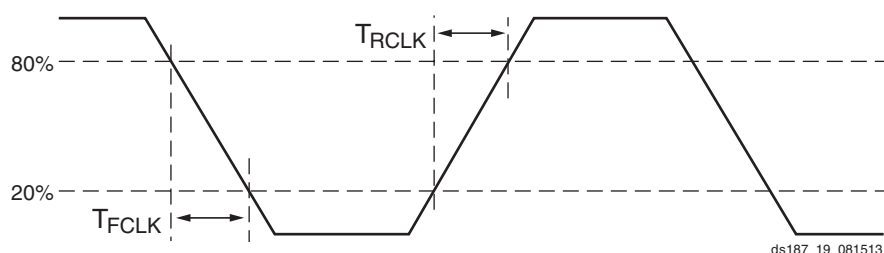
Figure 19: Reference Clock Timing Parameters
