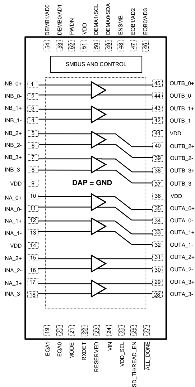
Figure 1. DS125BR800 Pin Diagram 54 lead
