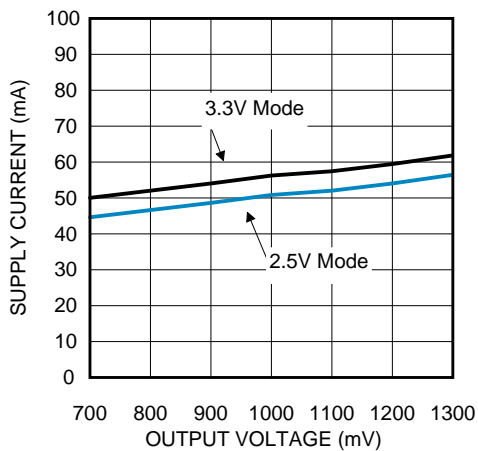
Figure 9. Supply Current vs. Output Voltage Setting
