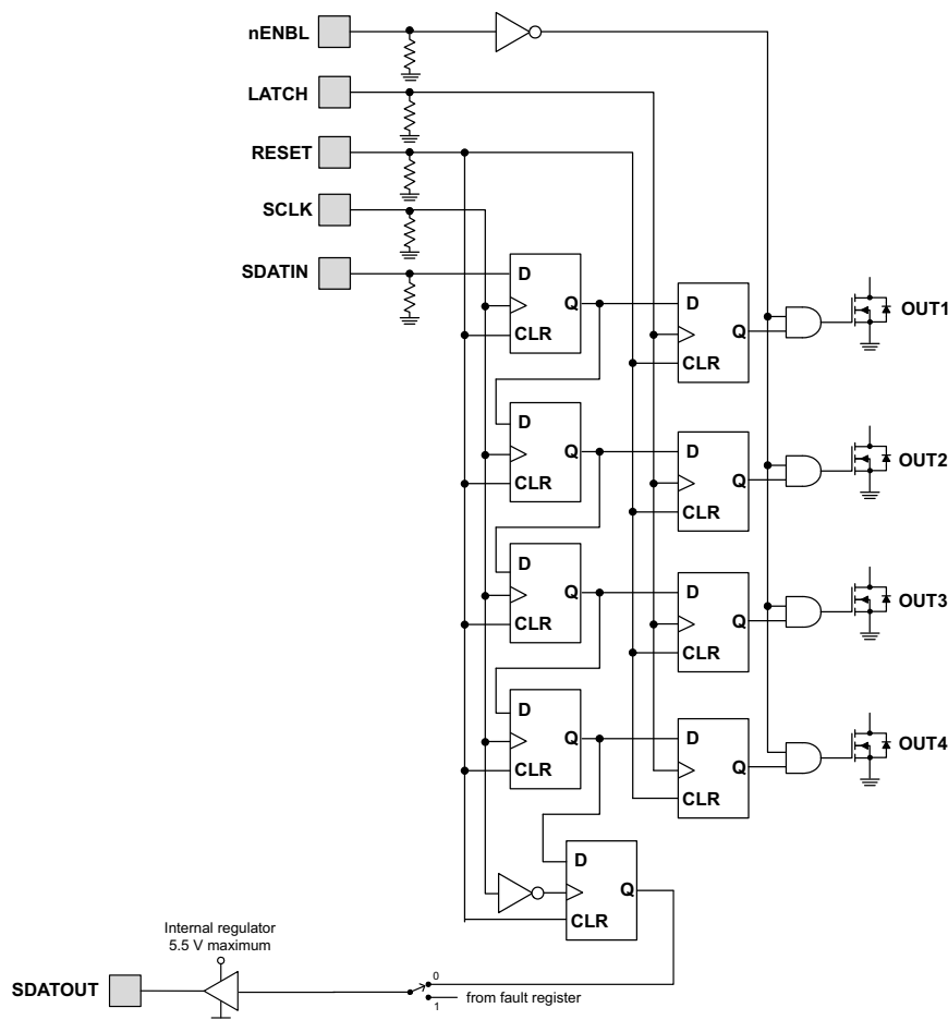
Figure 2. Serial Interface Operation
