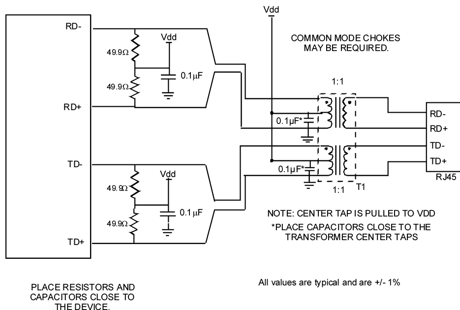
Figure 9-1. 10/100 Mb/s Twisted Pair Interface
