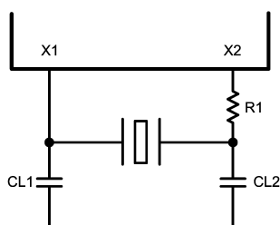
Figure 9-2. Crystal Oscillator Circuit
