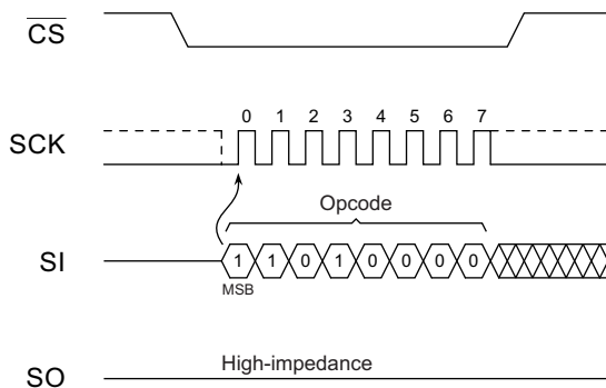
Figure 8-10. Program/Erase Resume
