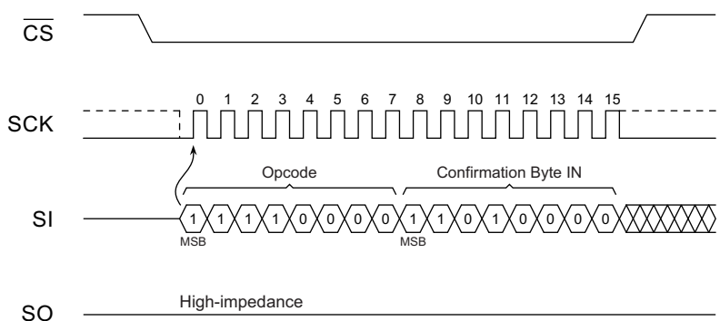
Figure 12-1. Reset
