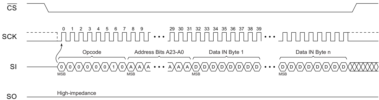
Figure 8-2. Page Program
