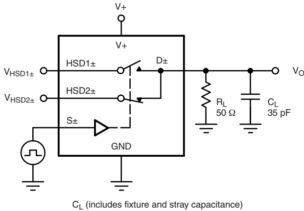
Figure 2. Break-Before-Make Interval
