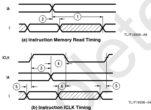
FIGURE 5-5. Instruction Memory Timing
