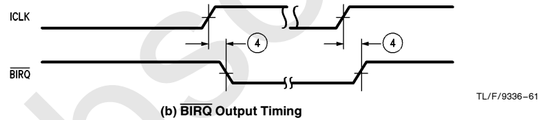
FIGURE 5-9. Interrupt Timing
