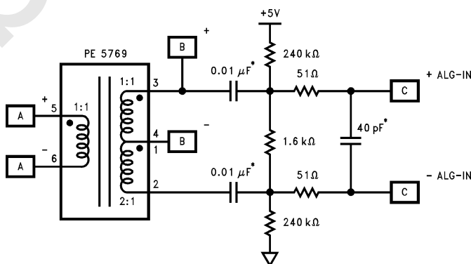
FIGURE 3-12. BCP Receiver Design
