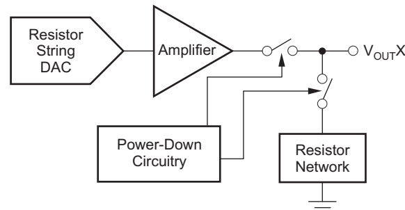
Figure 93. Output Stage
