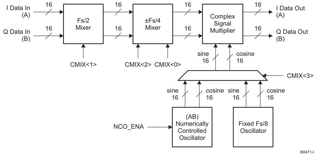
Figure 73. Path of Complex Signal Mixer
