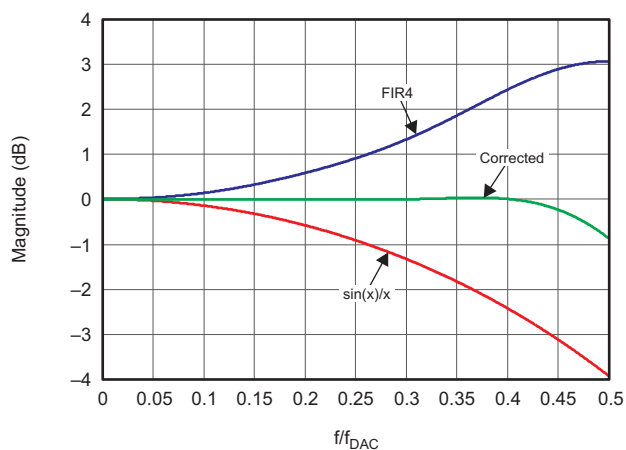
Figure 72. Magnitude Spectrum for Inverse Sinc Filter
