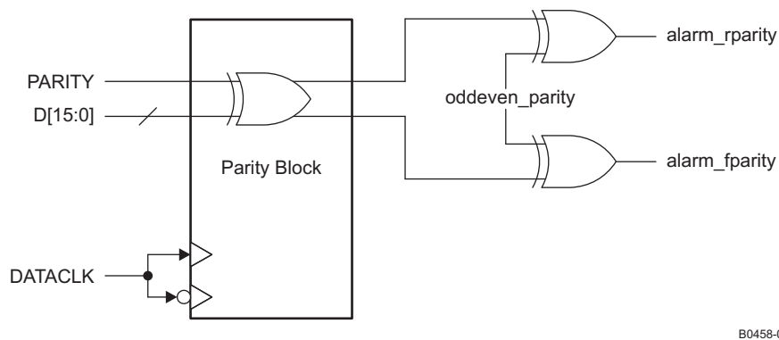
Figure 81. DAC3484 Word-by-Word Parity Check
