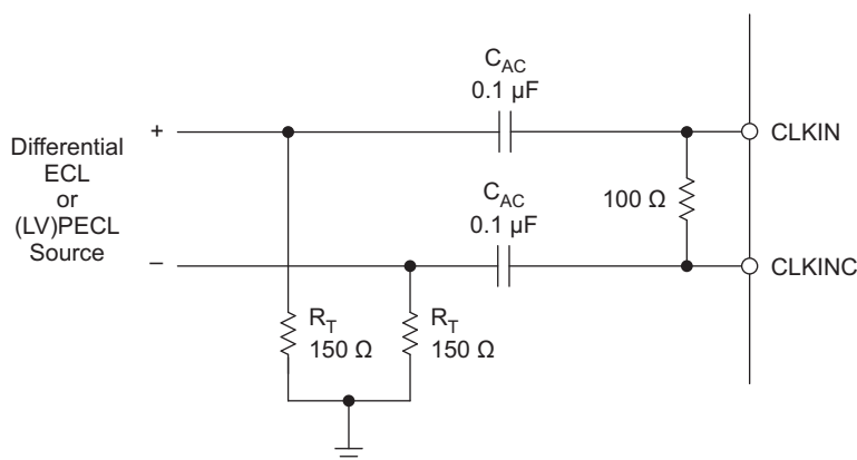
Figure 84. Preferred Clock Input Configuration with a Differential ECL/PECL Clock Source
