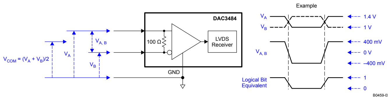
Figure 86. LVDS Data Input Levels
