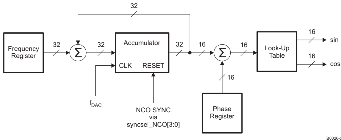
Figure 74. NCO Block Diagram
