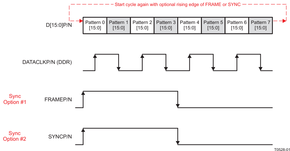
Figure 79. IO Pattern Checker Data Transmission Format
