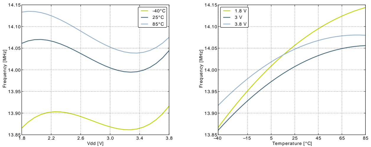
Figure 3.10. Calibrated HFRCO 21 MHz Band Frequency vs Temperature and Supply Voltage
