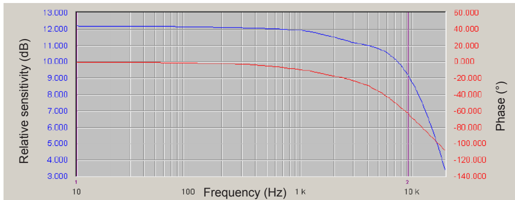
Figure 1: Frequency response
