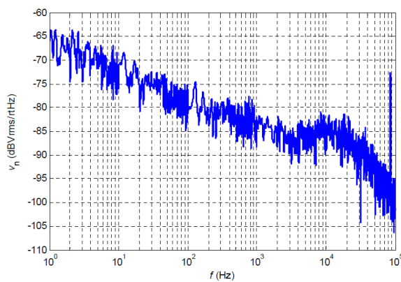
Figure 2: Output noise, spectral density
