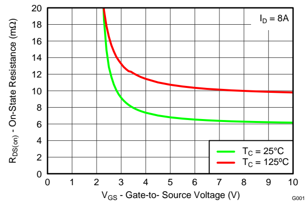
Figure 20. Sync MOSFET R_{DS(on)} vs V_{GS}
