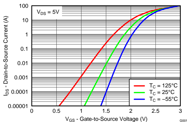
Figure 12. Sync MOSFET Transfer
