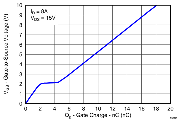
Figure 14. Sync MOSFET Gate Charge
