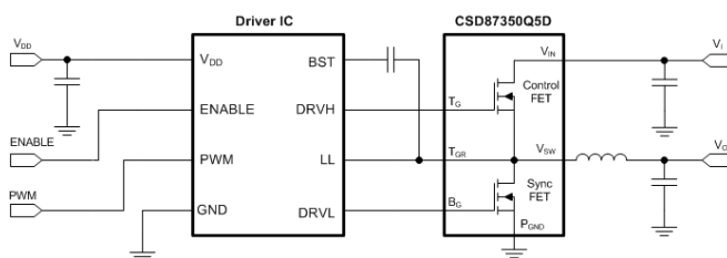
TYPICAL CIRCUIT
